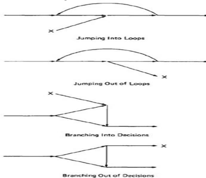
Figure 5.8: Un-structured sub-graphs.
