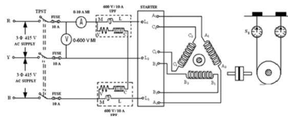
Circuit – 13
