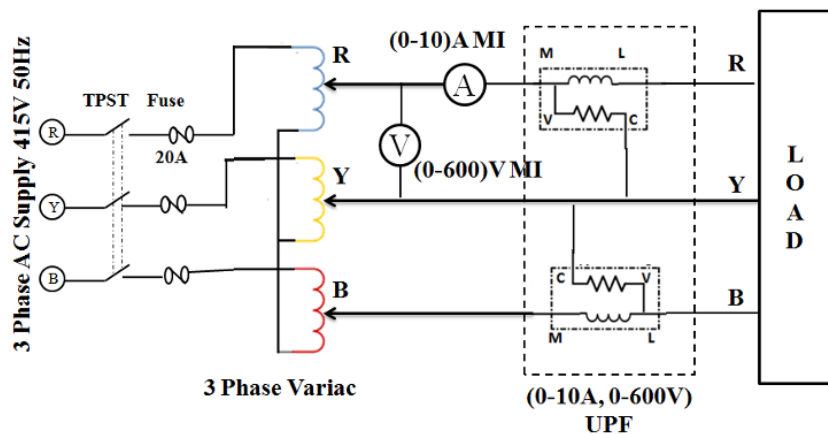
Circuit – 11
