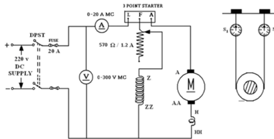
Circuit – 12
