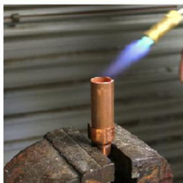
Fig.9.3 Hard soldering of copper with brass
