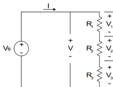
Circuit – 4
