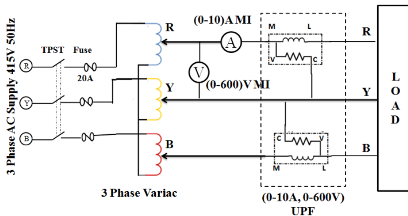
Circuit – 11
